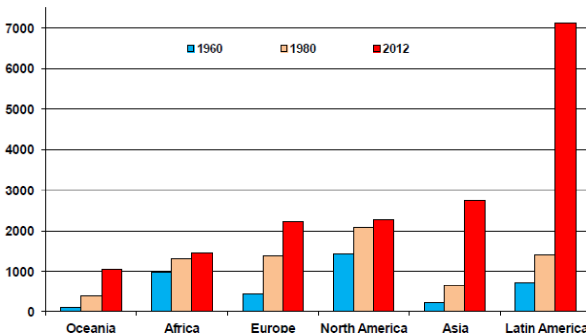
Copper Mine Production by Region, 1960, 1980 & 2012 (Thousand metric tonnes) Source: ICSG
